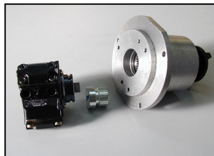
Motoring coupling P.N.: CDAG0115-00
